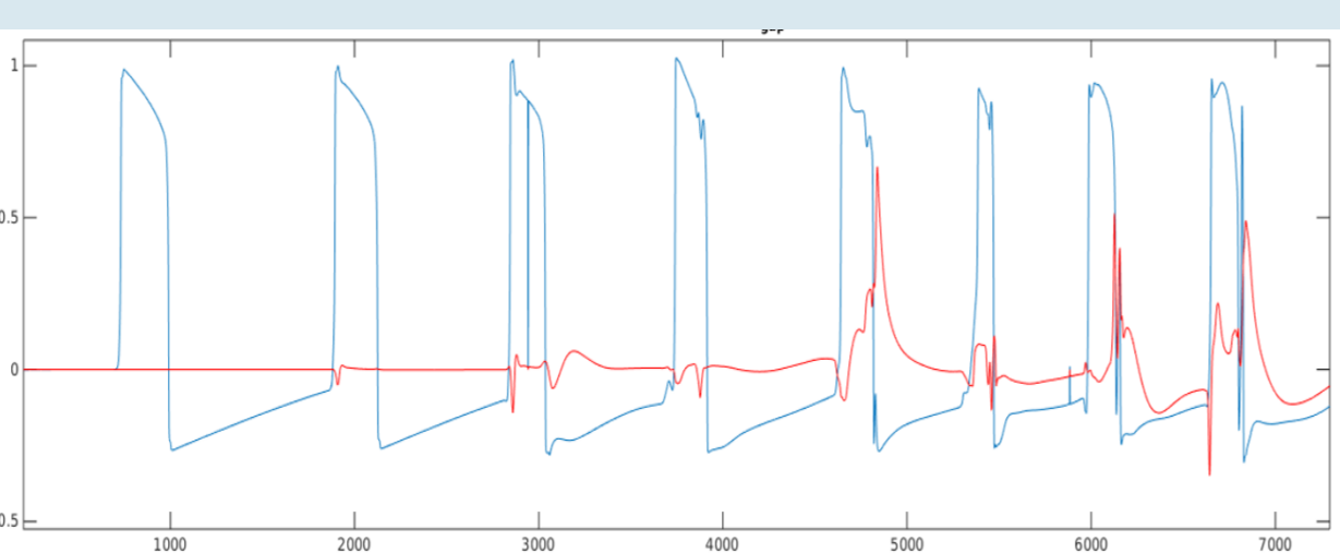
Figure 8 : Illustration of bound charges (red) inhibiting membrane currents, which process alters action potentials (blue).
