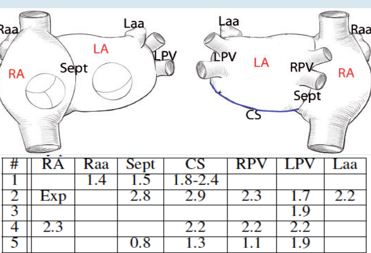
Figure 6 : Table of the measured Fisher exponents for 5 patients. It appears that regional gradients may indicate a source of activity.
