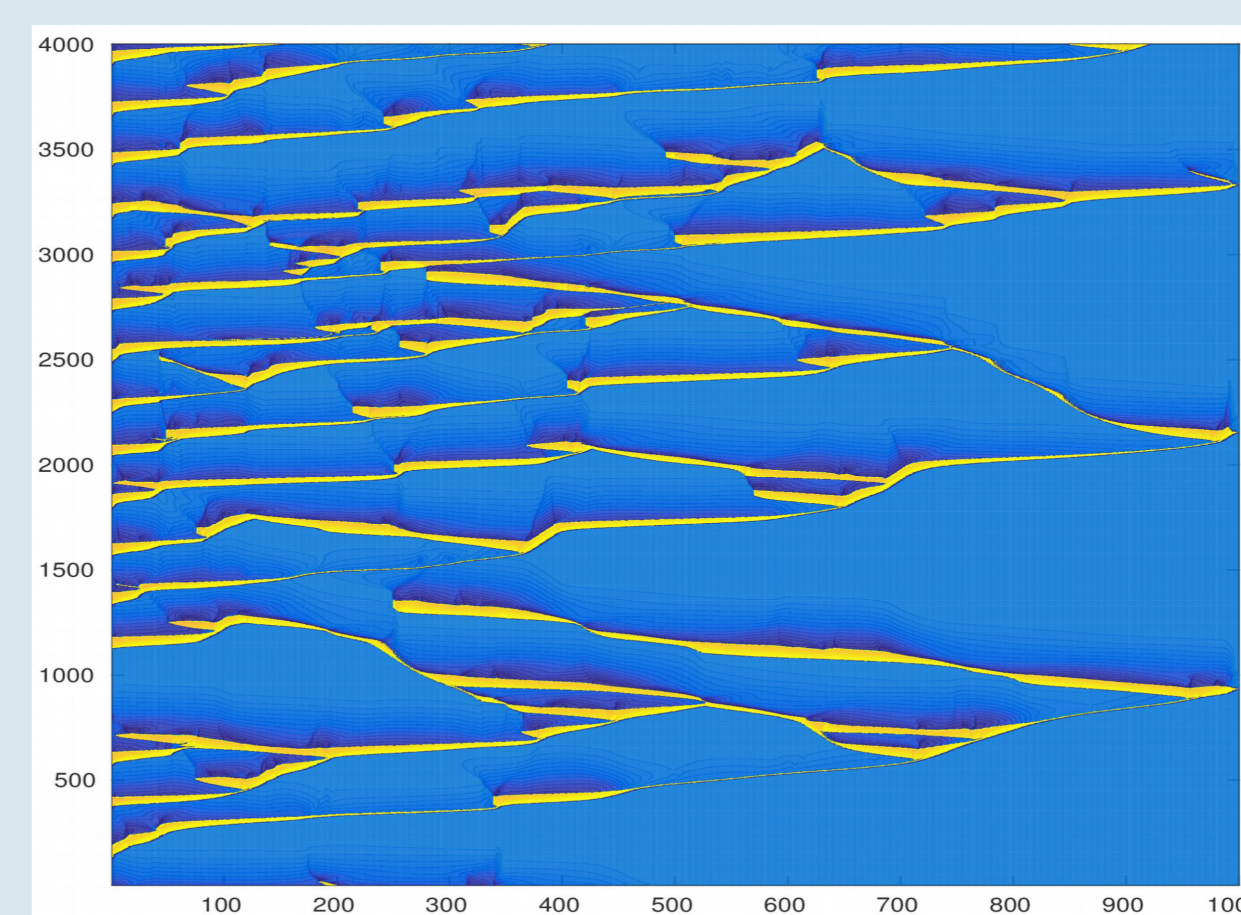
Figure 10 : Spatio-temporal map of the membrane potential showing many back-scattering events, some abnormal automaticity, and an overall hierarchical branching propagation.
