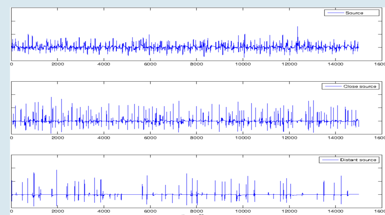
Figure 9 : Instance of three traces of the gap junction flux divergence near, at mid distance, and far from the boundary source. Fisher exponents decrease gradually with the distance from the source.
