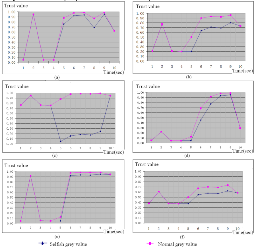
Figure 6 Different weight vectors (attack strategy detected in (c))
