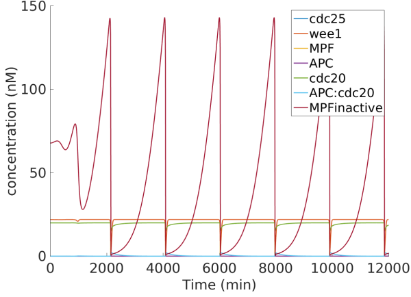
Fig. 3. Oscillations of the components of the cell cycle model. Parameters: wee1_{TOT} = 22.0 , cdc25_{TOT} = 20.0 , APC_{TOT} = 40.0 , cdc20_{TOT} = 20.0 , \gamma_1 = 3.0 , \gamma_2 = 0.1 , V_1 = 0.1 , k_1 = 7.6 , V_2 = 2.5 , k_2 = 7.6 , V_3 = 0.5 , k_3 = 5.4 , V_4 = 5.0 , k_4 = 4.3 , V_5 = 70.0 , k_5 = 50.0 , V_6 = 20.0 , k_6 = 50.0 , V_7 = 0.1 , k_7 = 10.2 , V_8 = 1.0 , k_8 = 10.5 , V_9 = 1.5 , k_9 = 50.6 , V_{10} = 0.5 , k_{10} = 60.1 , V_{AC} = 0.2 , V_{CA} = 0.15 and S_{GF} = 0.24 . Units for V_1, V_4, V_5, V_6, V_7, V_{10} and V_{CA} are min^{-1} for V_2, V_3, V_8, V_9 and S_{GF} are nM.min^{-1} , for \gamma_1, \gamma_2 and V_{AC} are min^{-1}.nM^{-1} and for all k 's are nM .
