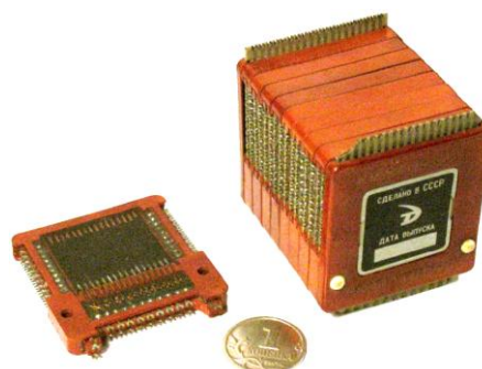
Figure 4. "Cub-2" - The module RON in capacity of 16 19-digit words, "Cub-2" in capacity of 128 19-digit words, Between them a coin 1 copeck 2003) The size of the module 32x34x4,125 mm. The size of the block: 128x19 bats – 32x34x42 mm 256x19 bats – 32x34x42 mm Such a Cub flined around of the Moon.
