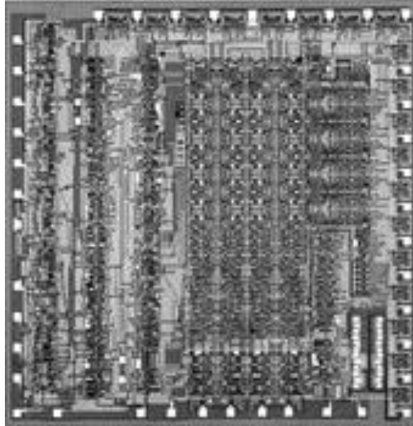
Figure 7. Topology K587IK2
