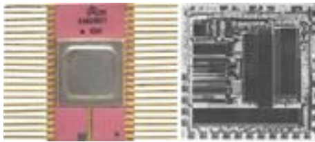
Figure 17. K1801VE1 in the package (full-scale) and its topology.
