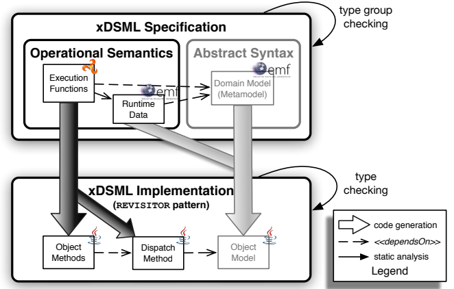
Fig. 2: Approach overview
