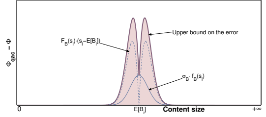
Figure 2: Error introduced by \Phi_{qac}(\mathbf{x}, \mathbf{y}) in Lemma 4.7 for a fixed value of \mathbb{E}[B_i] .
