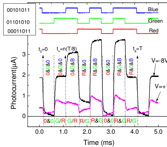
Fig. 3 Multiplexed signals under reverse and forward bias. On the top, the optical signal used to transmit the information guide the eyes on the different ON-OFF states. The recovered bit sequences are shown as an insert.
