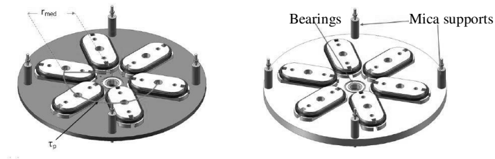
Fig. 3. Final aspect of T1 (left) and T2 (right) semi-stators design.
