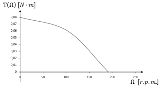
Fig. 9. Experimental torque/speed characteristic for topology T1.
