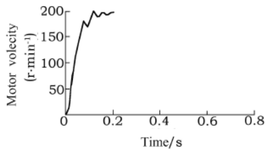
Fig. 4. Simulation results of system response to step signal
