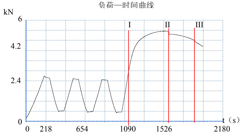
Fig.6. Loading-time Curve
