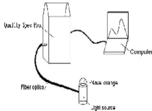
Fig.1. Vis-NIRs system
