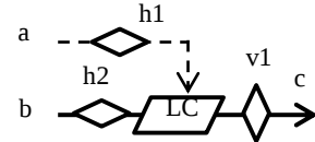
Figure 4 A_{17}(3) corresponding to BT_{17}(3)
