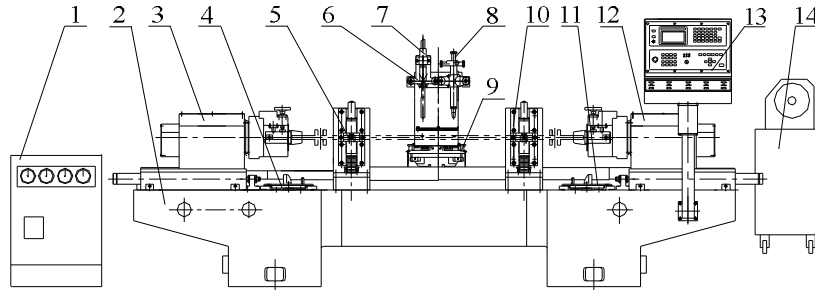
1 hydraulic system; 2 machine tool bed; 3,12 drive box; 4,11 bracket; 5,10 clamping device; 6 automatic cutting and welding device; 7 welding torch; 8 cutting gun; 9 moving workbench; 13 numerical control system; 14 welding controller.
