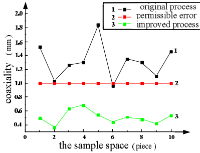
Fig.10. Curve diagram of coaxiality under different process conditions
