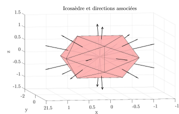
Figure 3: Maillage directionnel
