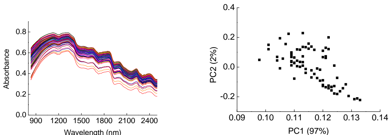
Fig. 2. The PCA score plot of chicken manure
