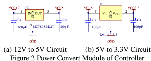
Figure 2 Power Convert Module of Controller
