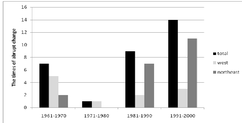
Fig. 6. The times of abrupt change detected by the Sliding t -test ( n_1=n_2=10 ) in different decades.
