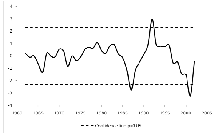
Fig. 4. The abrupt change tested by the Sliding t -test for annual precipitation series in Youyu station from 1962 to 2002 ( n_1=n_2=5 ).
