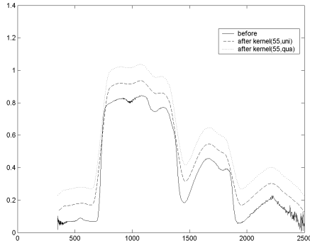
Figure 3. Kernel smooth
