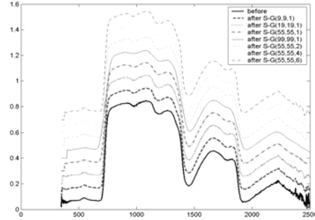
Figure 2. S-G smooth
