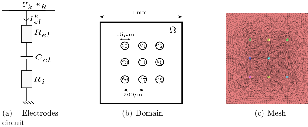
Figure 2: Schematic representation of the electrodes electrical circuit (a). 2D domain \Omega with dimensions and positions of the 9 electrodes (b). Computational mesh representing a triangular discretization of the domain \Omega with h \approx 25 \mu\text{m} (c).
