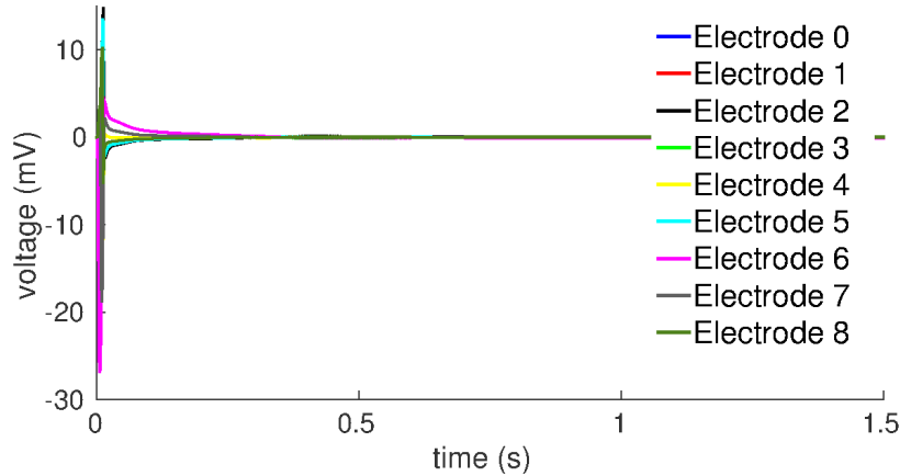
Figure 3: Simulated field potentials over the 9 electrodes for ventricular-like hiPSC-CM without introducing any heterogeneity in the model.
