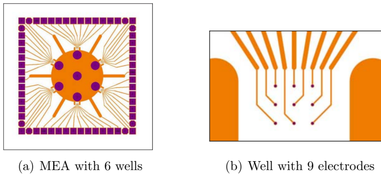
Figure 1: Multichannel Systems device [19]. Panel (a): 60-6well MEA device. Panel (b): zoom on one well with the 9 electrodes (reproduced with permission).
