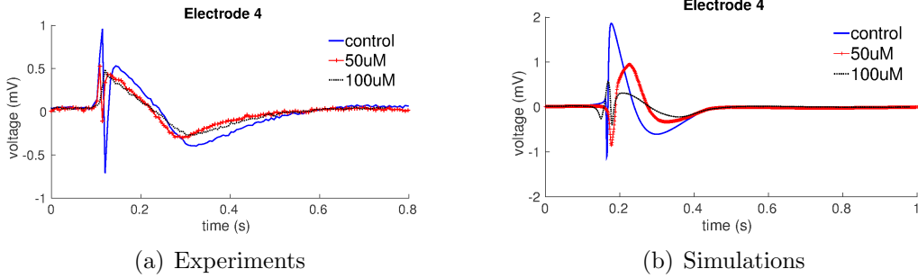
Figure 14: Comparison of the field potential between control conditions and 50µM and 100µM of mexiletine for one beat: experimental measurements (a) and simulations results (b).
