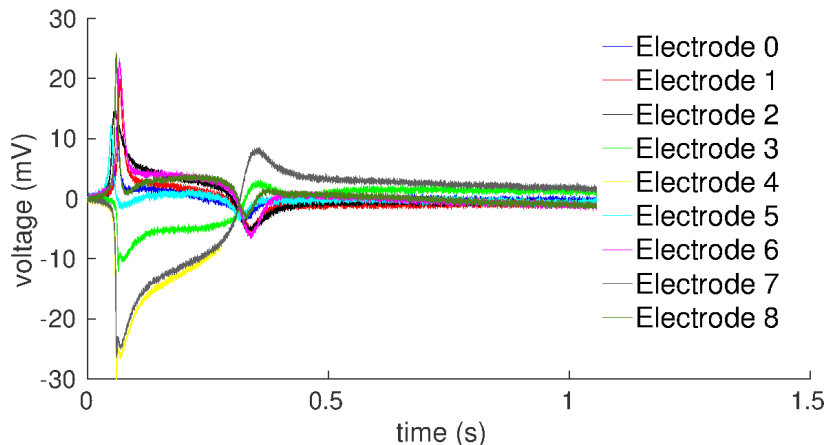
Figure 4: Field potential signals of the 9 electrodes recorded from one MEA well. The experimental measurements were produced by Janssen / NMI and provided by Notocord .
