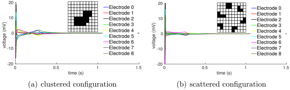
Figure 11: Field potential shapes obtained with F = 20\% , with two different spatial arrangements (the black part is \Omega_2 ): on the left results for a “clustered configuration”, on the right results for a “scattered configuration”.
