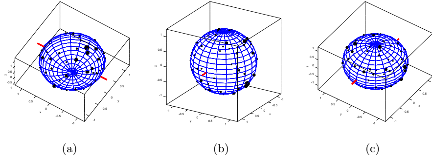
Fig. 4: Sample acquisition scheme obtained with our method for the Watson’s dispersed stick with SNR=20. The main orientation of the sticks is plotted with the red line. The black dots represent q -space locations. The sizes of dots are proportional to the magnitudes of gradient G . Note that the regions located perpendicular to the main orientation of sticks are covered most densely and the G -values are the highest there. On a contrary, the regions located parallel to the orientation are covered more loosely and the G -values are visibly lower.
