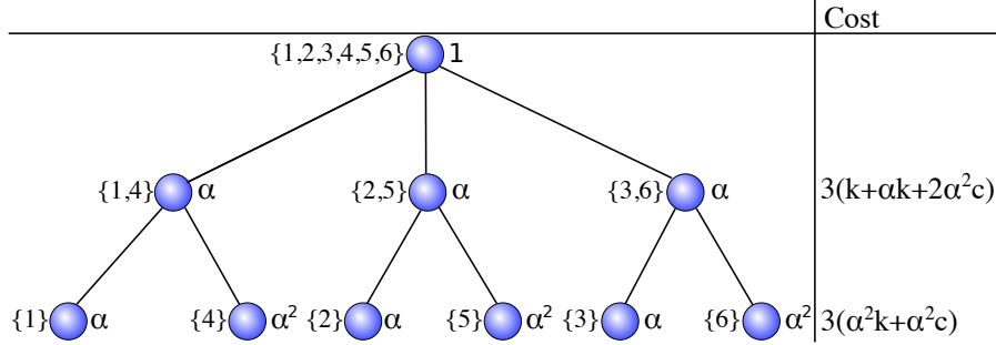
Figure 1: A ternary dimension tree for \mathcal{X} . The \mu set of the node is provided on the left, and the tensor size coefficient is provided on the right of each tree node. The TTM cost of each level is provided on the right.
