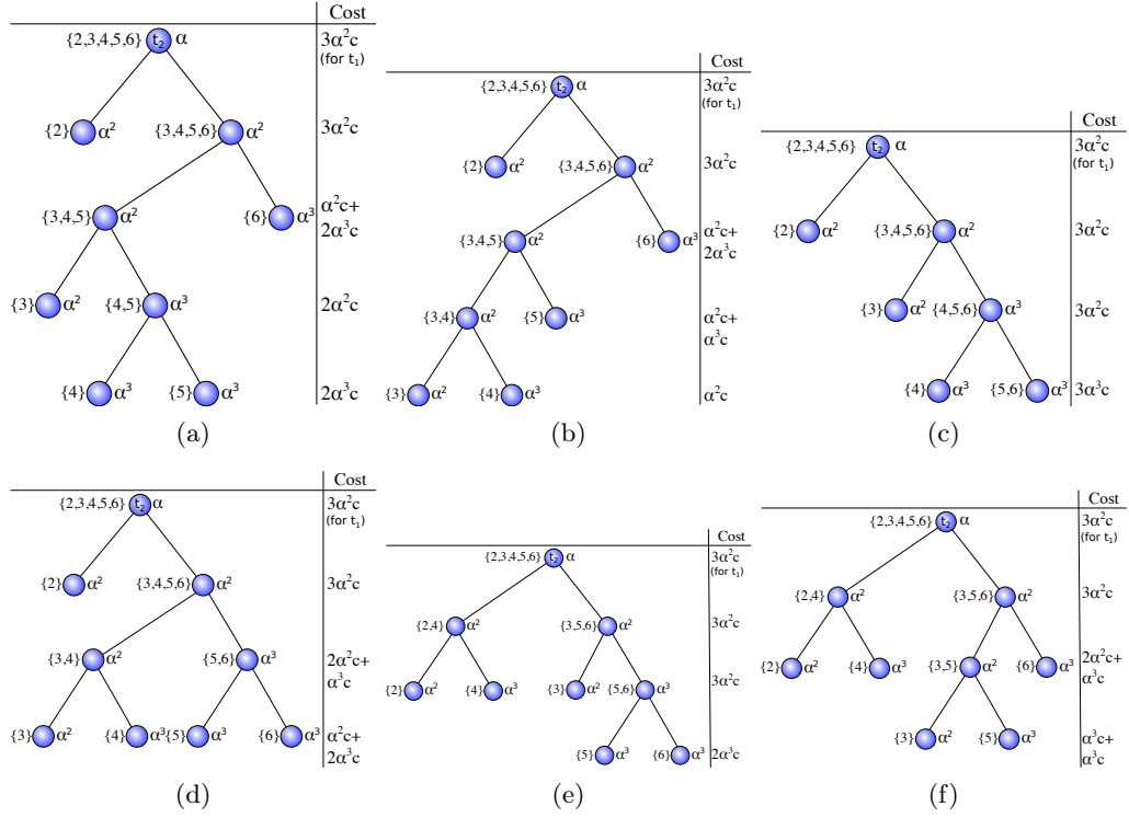
Figure 2: All possible configurations and associated TTM costs at each level of BDTs rooted at t_2 . \mu(t) is given on the left of each tree node t . On the right of a tree node, the size coefficient of its tensor is provided, i.e., t_2 has a tensor of size (I_1 I_2 I_3 I_4 I_5 I_6)\alpha .
