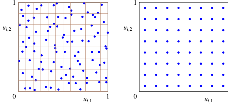
Fig. 1 An illustration of stratified sampling (left) and a midpoint rule (right) over (0, 1)^2 .
