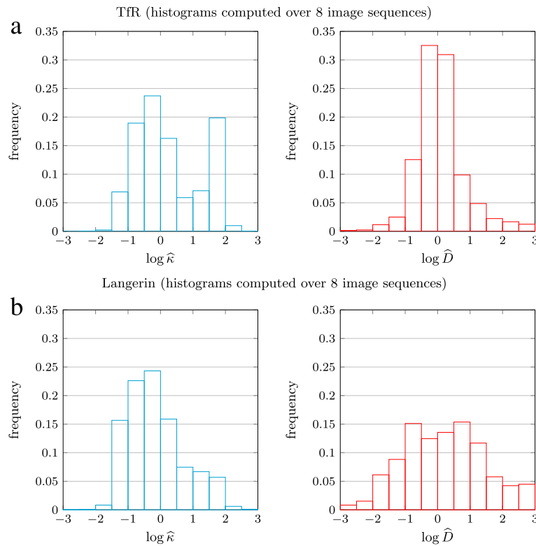
Fig. 5 Comparison of the histograms of the biophysical parameters \kappa and D estimated respectively in 8 TIRFM image sequences depicting TFR (a) and in 8 TIRFM image sequences depicting Langerin (b)
