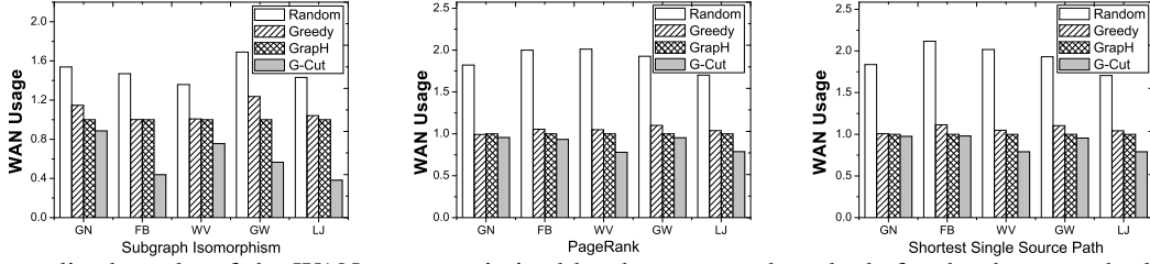
Fig. 6: Normalized results of the WAN usage optimized by the compared methods for the three graph algorithms.
