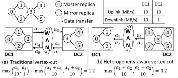
Fig. 2: A comparison between two graph partitioning methods: (a) traditional vertex-cut and (b) heterogeneity-aware vertex-cut. Widths of the up/down links indicate network bandwidths.
