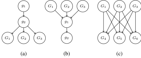
Figure 1: Example M-SPG structures ( g_1 and g_2 are atomic tasks whereas G_1 to G_6 are M-SPGs): (a) fork: (g_1 \vec{;} g_2) \vec{;} (G_1 || G_2 || G_3) ; (b) join: (G_1 || G_2 || G_3) \vec{;} (g_1 \vec{;} g_2) ; (c) bipartite: (G_1 || G_2 || G_3) \vec{;} (G_4 || G_5 || G_6) .
