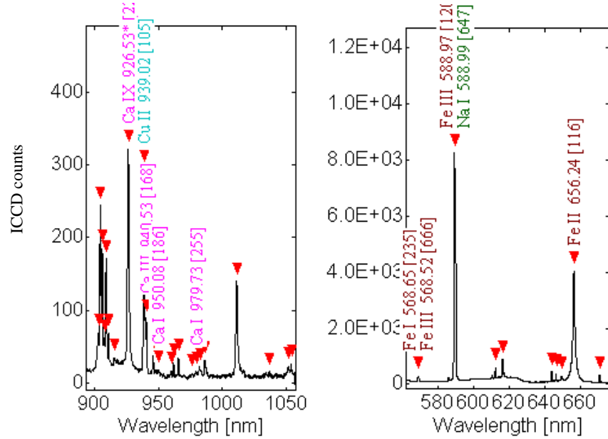
Fig. 2. Typical LIBS spectra of Ca, Cu, Fe, Na in pericarps
