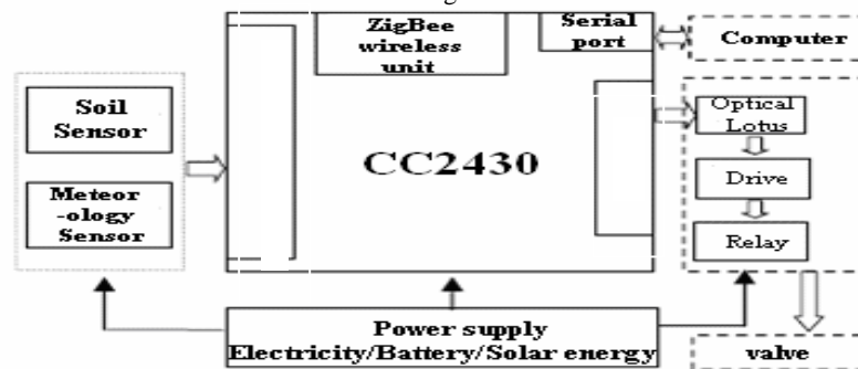
Fig.1 System diagram
