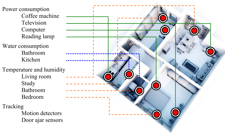
Fig. 2. Domestic sensors
