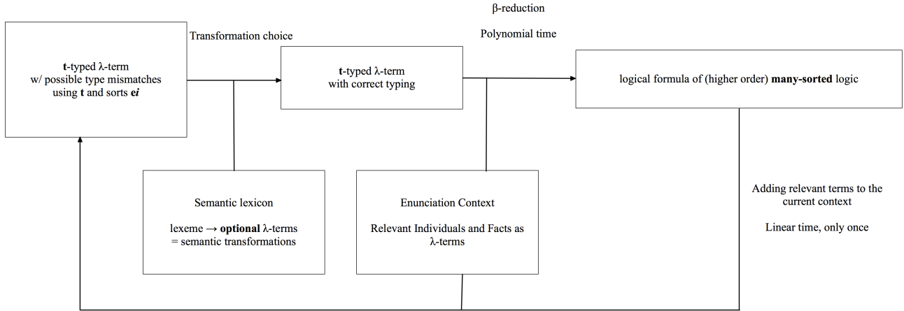
Fig. 3. Parsing-Knowledge Representation Feedback
