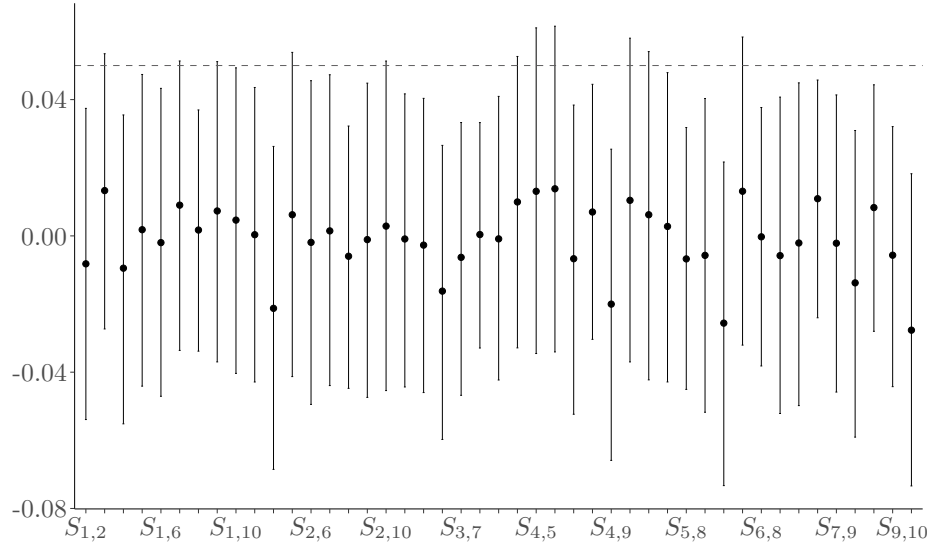
Figure 5: Plot of second-order Sobol' index estimates for the wing weigth function. The vertical bars represent the bootstrap confidence intervals. The horizontal dotted line marks the threshold (0.05).
