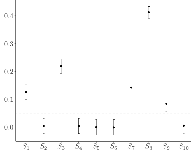
Figure 5: Plot of second-order Sobol' index estimates for the wing weigth function. The vertical bars represent the bootstrap confidence intervals. The horizontal dotted line marks the threshold (0.05).
