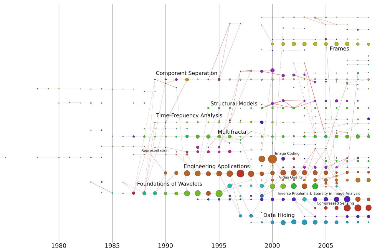
Figure 3: Overview of the history of wavelets. Streams are labelled according to the subfield within wavelets development (see text for details). Zoomable version available at
