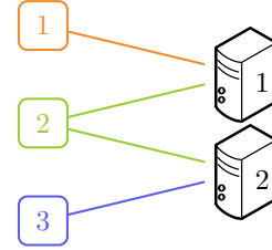
Fig. 1. Bipartite graph of compatibilities. The cluster contains two computers. There are three job classes, one for each possible assignment: class-1 and 3 jobs can only be served by computers 1 and 2, respectively, while class-2 jobs can be served by both computers.
