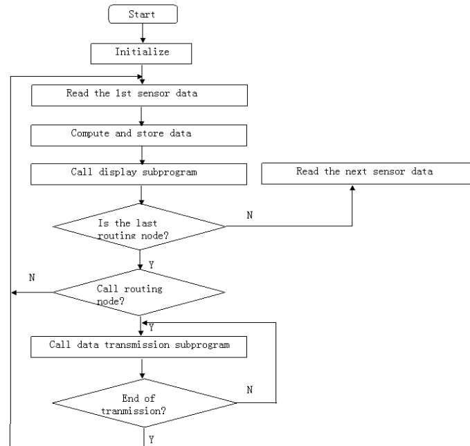
Fig.3 Main program flowchart of terminal node
