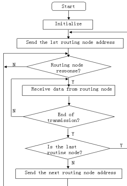
Fig.2 Main program flowchart of the center node
