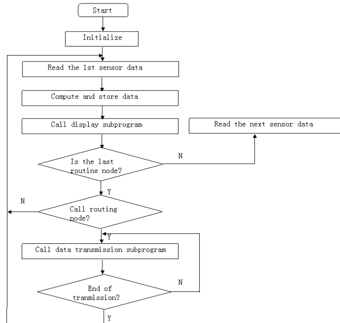
Fig.3 Main program flowchart of terminal node
