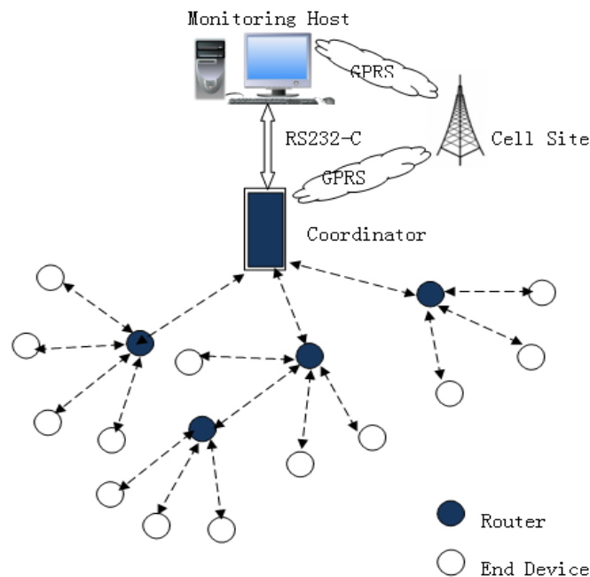
Fig.1 Overall structure
