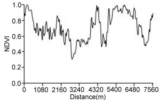
Fig. 3. NDVI changing condition of GGGC-W
