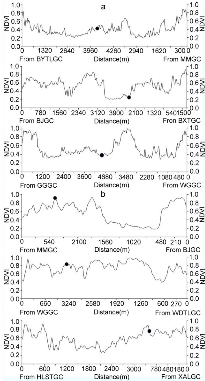
Fig. 4. NDVI changing trend between 2 adjacent rural settlements for the first condition and the second condition
