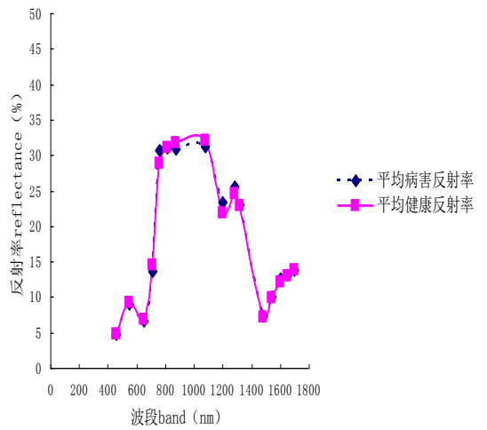
Fig.4. Reflectance spectrum of Brassica napus leaves under the background of field groups 17 days after finish flowering (5.3)
