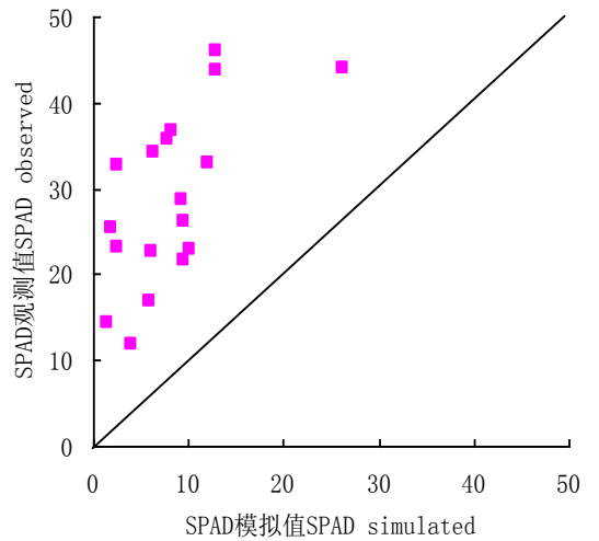
Fig. 16 Comparison of observation and simulation in SPAD value of different diseases
