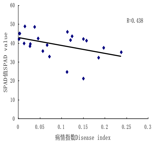
Fig.10. Relationship between SPAD value and DI
