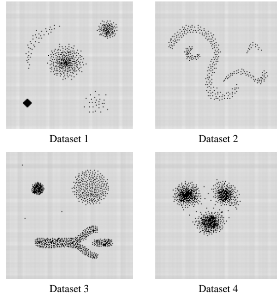
Fig. 3. Sample datasets
