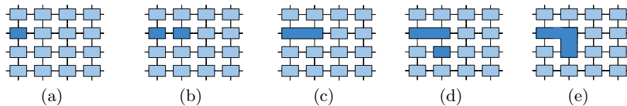
Fig. 1. Merging process: For a given tile (a), at a given step, one of its neighbors is considered as a candidate for merging (b). Their similarity is above the given threshold S , thus they are merged (c). At another step, a neighbor of the new tile is considered as a candidate for merging (d). Their similarity is above S , thus, they are merged (e).
