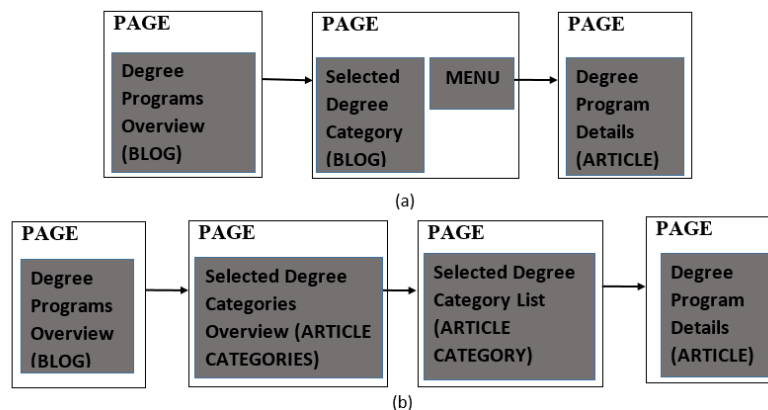
Fig. 6. An example of a domain functionality design pattern.
