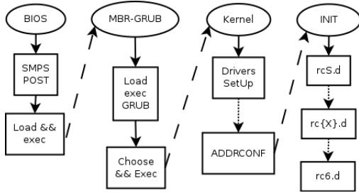
Figure 1: Linux monitored boot sequence.
