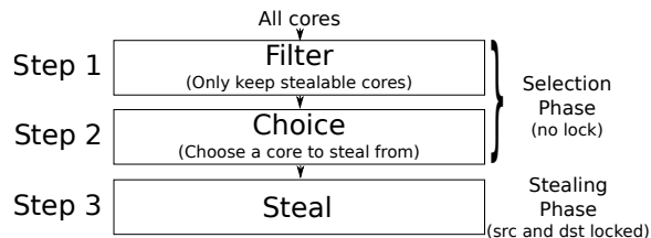
Figure 1: The three steps performed by a core during a load balancing round. First, the core decides from which cores threads can be stolen. Second, the core decides from which core to steal amongst the selected cores (if any). Third, the core performs the stealing operation. During the third step, the runqueue of the core that initiated the stealing operation and the runqueue of the targeted core are both locked.
