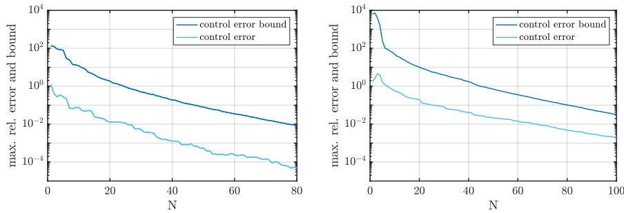
Fig. 4 Maximum relative control error and error bound over number of Greedy iterations N for strong-constraint case (left) and weak-constraint case (right).
