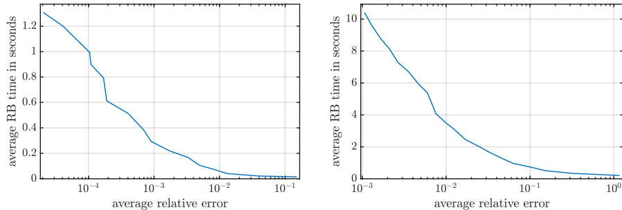
Fig. 5 Average online solution time of the reduced-order 4D-Var problem over the average relative error for strong-constraint case (left) and weak-constraint case (right).
