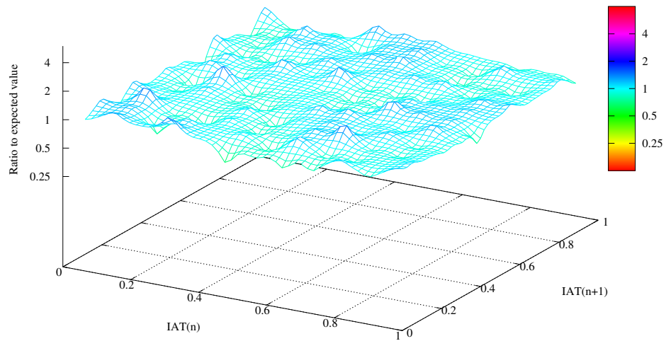
Figure 8: Lag plot for an EXP[\lambda] IAT log.
