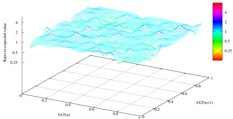
Figure 9: Lag plot for a WEIBULL[0.7, \lambda] IAT log.
