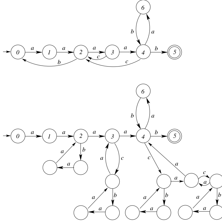
Fig. 2. A 1cfp dfa (up) and the corresponding balloon automaton (down).
