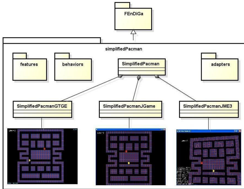
Fig. 4. The SimplifiedPacman game achitecture.
