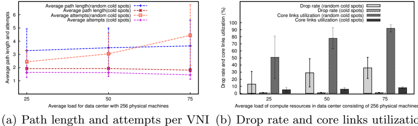
Fig. 7: Comparison between random cold spots and our default algorithm on 256 PMs.
