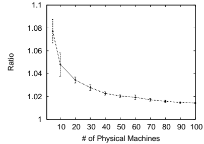
Fig. 6. Packing Ratio (Heuristic/Optimal)
