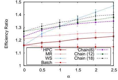
Fig. 8. Effect of energy fluctuation on workload cost
