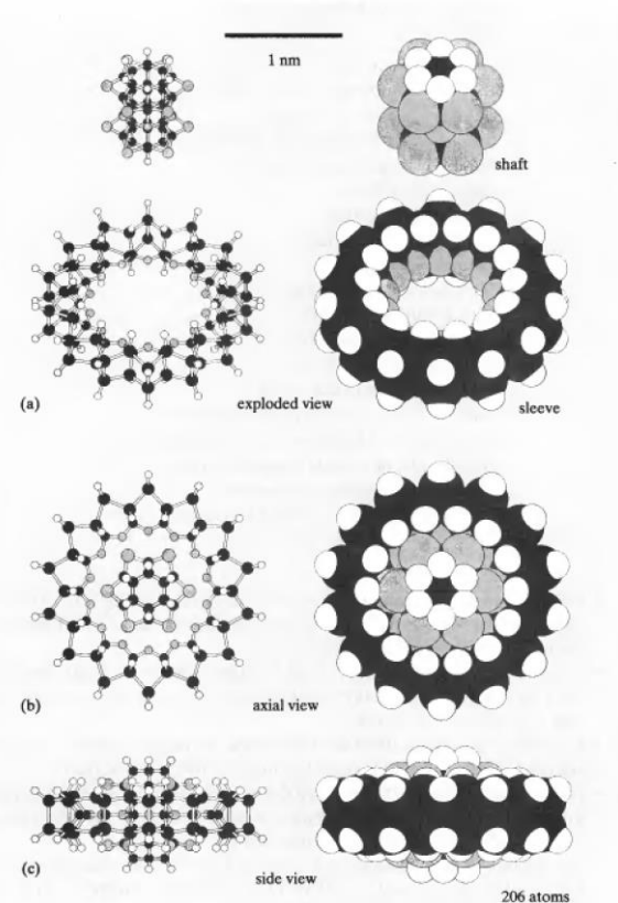
Nano-sized bearing (Drexler, 1992, p.4)
