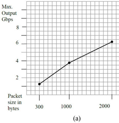
Fig. 2. Performance with and without references. (a) Throughput sensitivity to packet size (database result drives searchset selection). (b) Database result drives searchset selection. (c) Database result drives 2 nd database selection. © CloudShield Technologies, 2011
