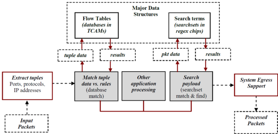
Fig. 1. Matching and searching operations on network packets.
